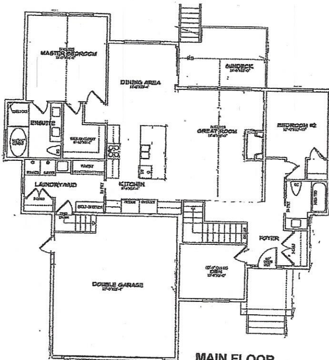
MAIN FLOOR 1585
