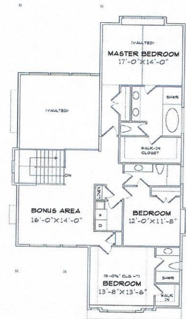
UPPER FLOOR PLAN 1558 SQ. FT.
