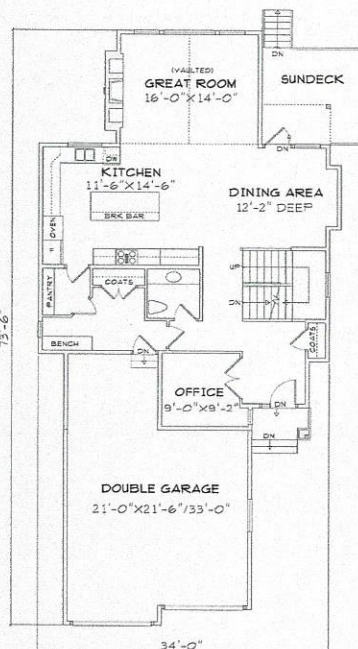
MAIN FLOOR PLAN 1295 SQ. FT.
