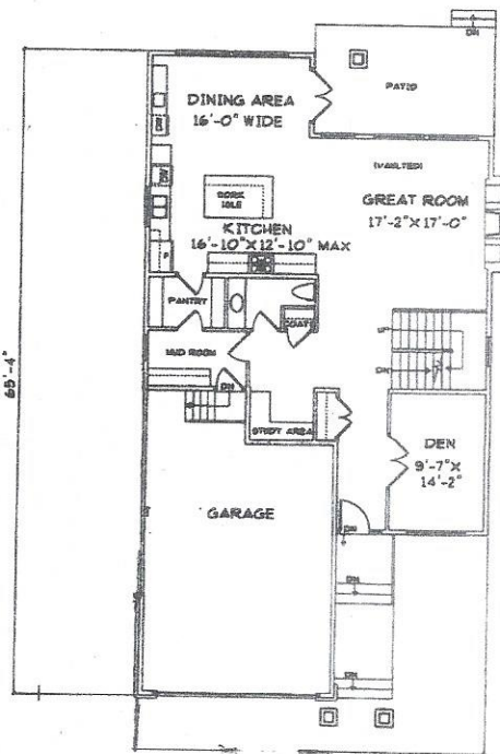
MAIN FLOOR PLAN 1357 SQ. FT
