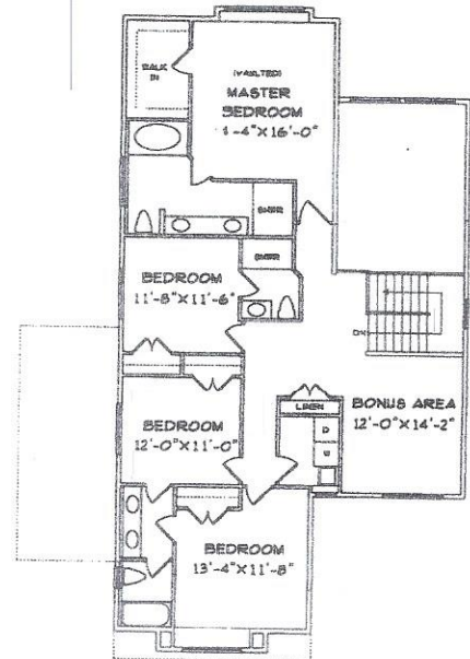
UPPER FLOOR PLAN 1577 SQ. FT.
