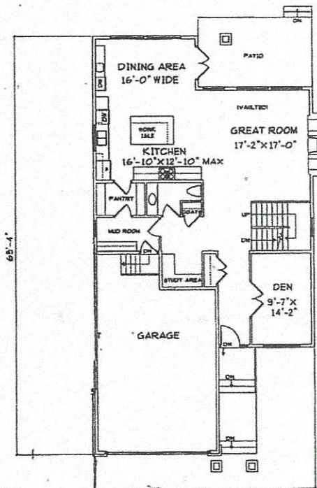
MAIN FLOOR PLAN 1357 SQ. FT
