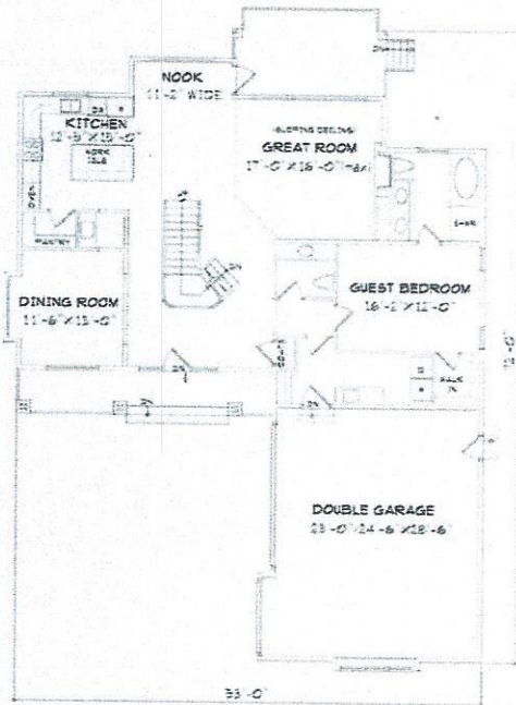
MAIN FLOOR PLAN 1761 SQ. FT.
