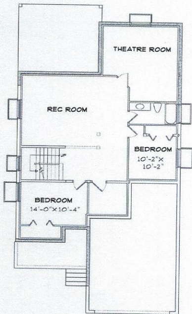
BASEMENT FLOOR PLAN 1432 SQ. FT.
